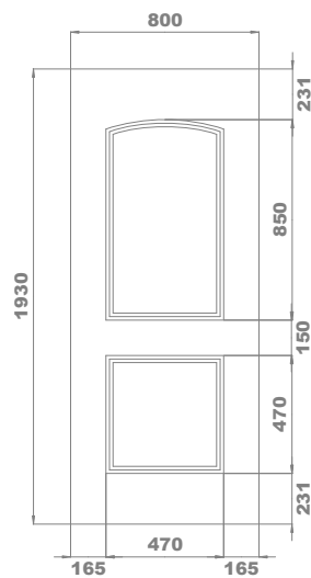
available as narrow panel with 470 moulding width - only available with G01, G02D & G02B
